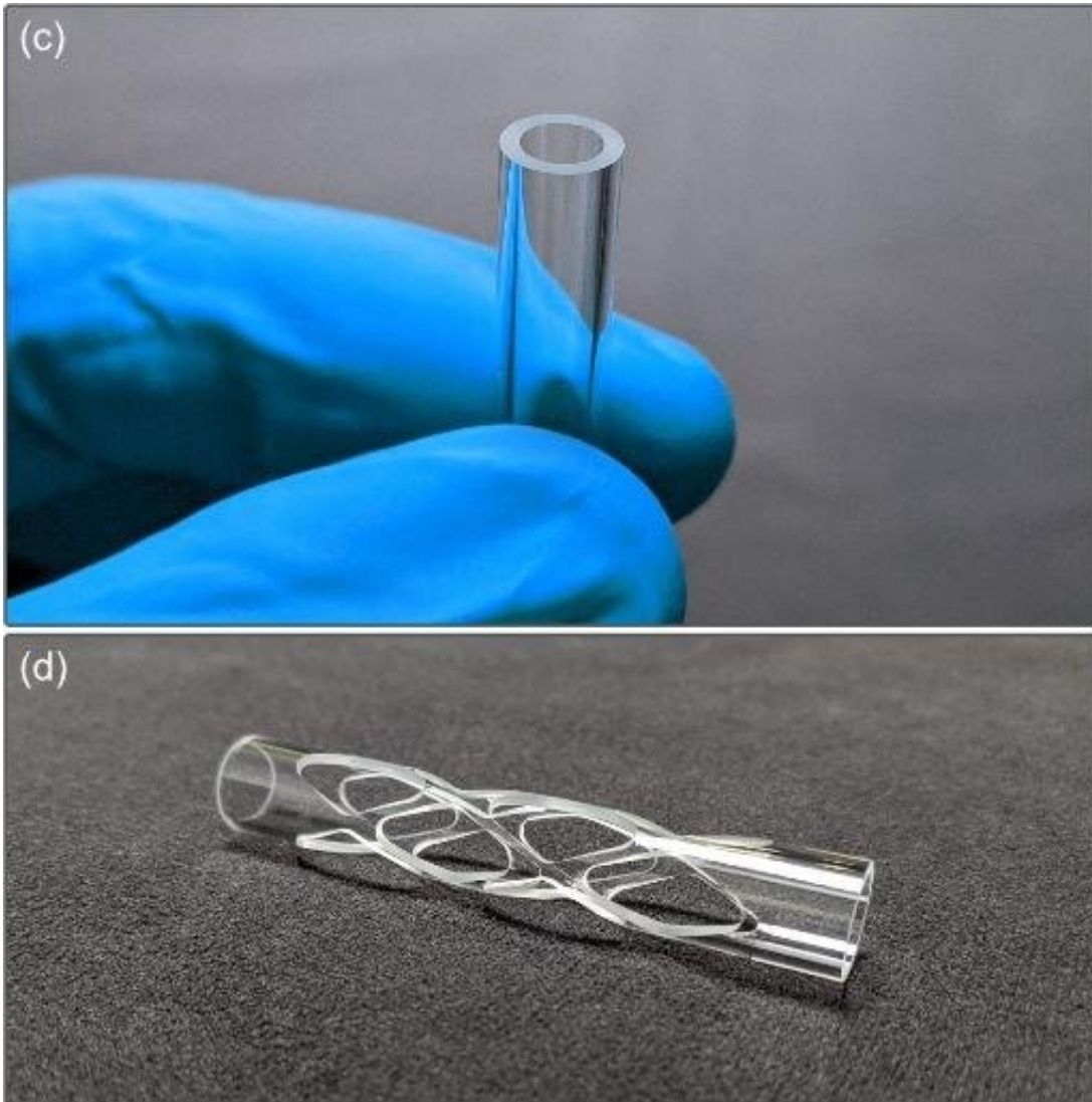
Cutting of glass tubes with complex inner and outer contours. Credit: Daniel Flamm et al.
