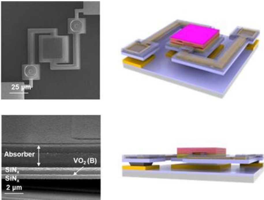
Electron microscope (left) and formula (right) of bolometer device. Credit: Korea Institute of Science and Technology (KIST)
