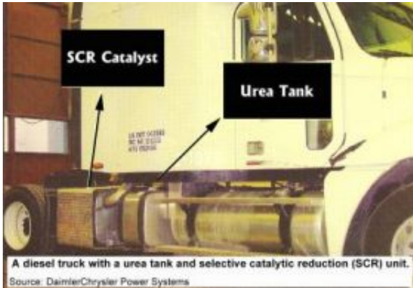
A prototype diesel truck with a urea tank and SCR unit. Credit: DaimlerChrysler Power Systems
