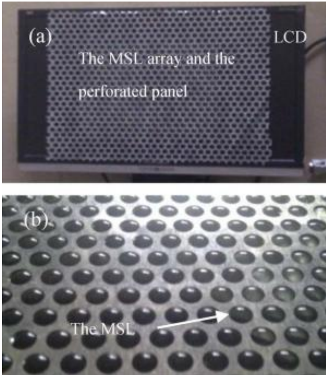
(a) Prototype of the proposed 3D display. (b) The microsphere lenses can project images to different spatial directions. Their larger curvature compared to planar lenses increases the viewing angle. Credit: Lv, et al. ©2015 IEEE
