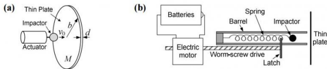
Conceptual sketches of: (a) impact transmitter; and (b) electromechanical pull-type actuator. Credit: arXiv:1507.01479 [physics.ins-det]
