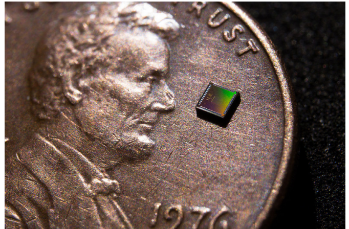
The temperature sensor is integrated into a small chip measuring 0.15 × 0.15 square millimeters in area. Credit: University of California - San Diego
