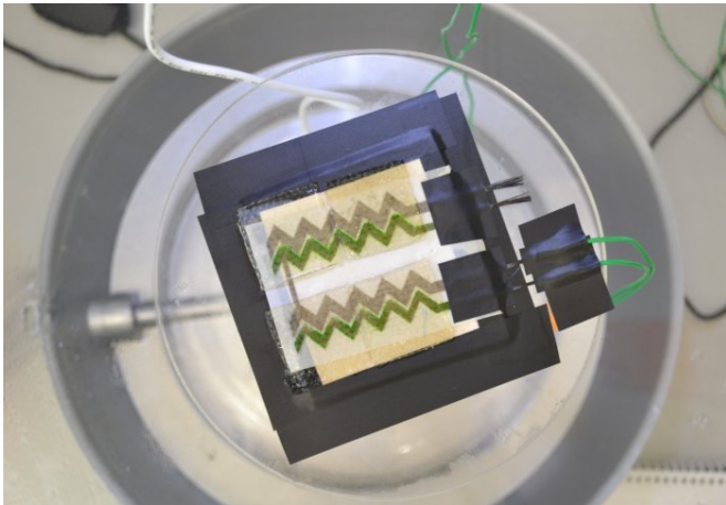
The wallpaper bio-solar panel. Credit: Imperial College London
