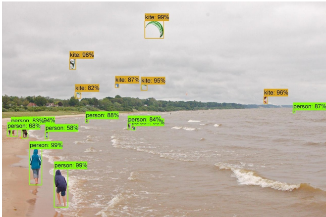
Example object detection using Faster-RCNN with NASNet. Credit: Google
