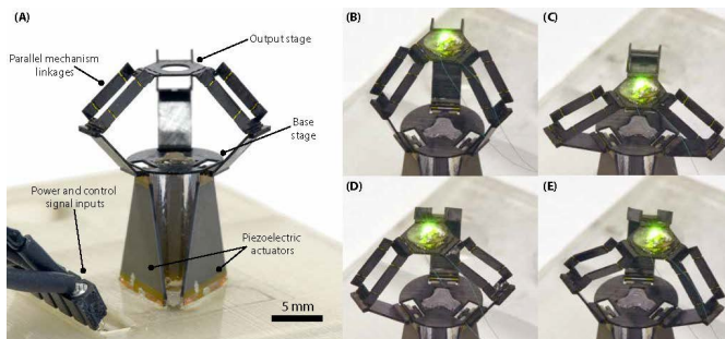
The milliDelta and its key components. Credit: McClintock et al., Sci. Robot. 3, eaar3018 (2018)
