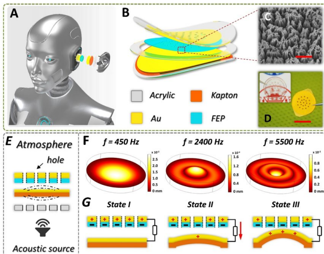
Structure and mechanism of the TAS. Credit: Hu et al.
