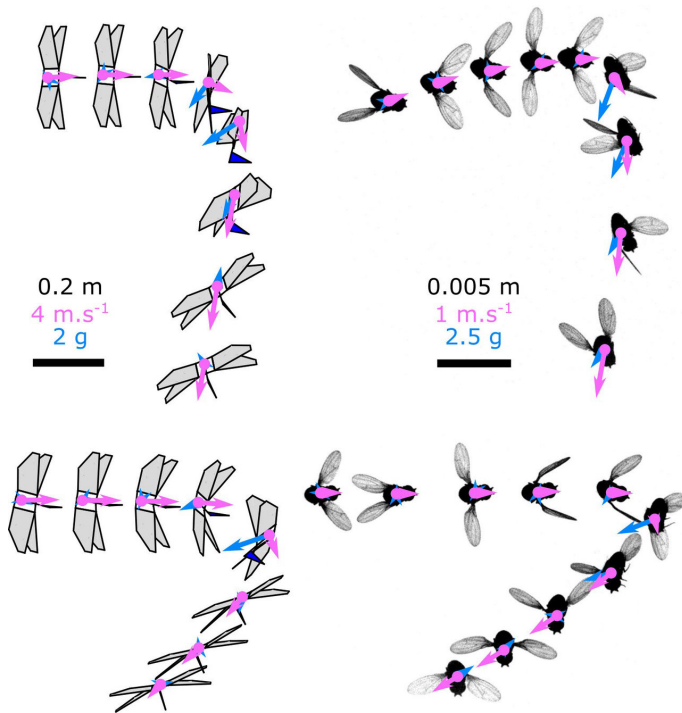
DelFly Nimble (left) performs rapid turns that closely resemble those of fruit flies when we try to swat them (right). Credit: TU Delft (CC BY-SA 4.0)
