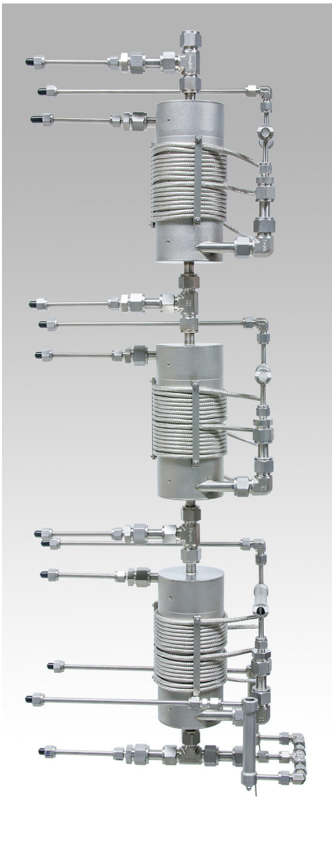
BIOGO high-pressure reactors for heterogeneous gas phase catalysis. Credit: Tobias Hang/Fraunhofer IMM
