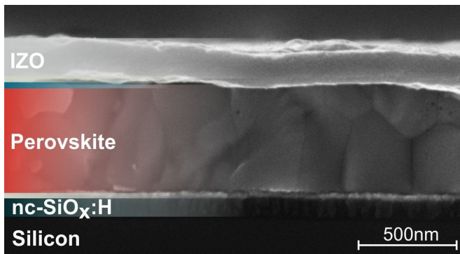
The SEM image shows the cross-section of a silicon perovskite tandem solar cell. Credit: HZB
