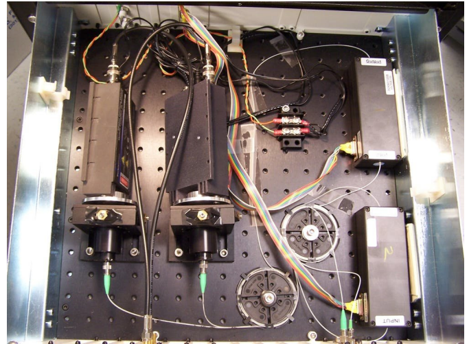
A look inside a prototype of the hardware that exchanges quantum cryptography keys. Credit: National Institute of Standards and Technology/Wikimedia Commons
