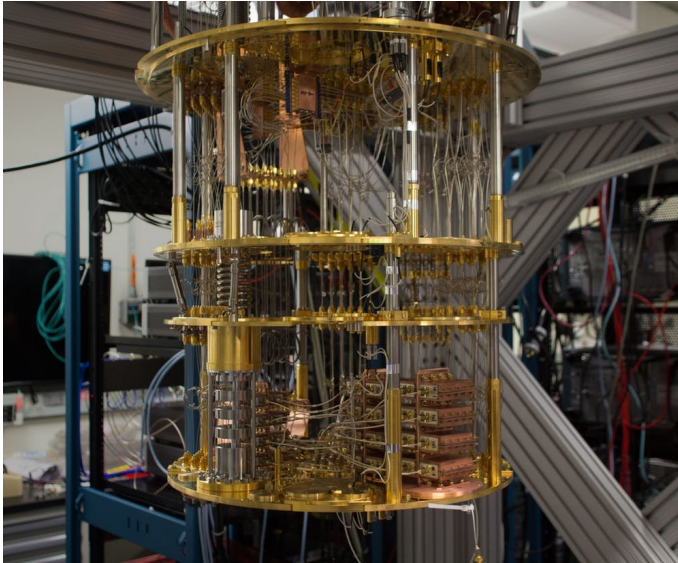
The insides of an IBM quantum computer. Credit: IBM Research , CC BY-ND
