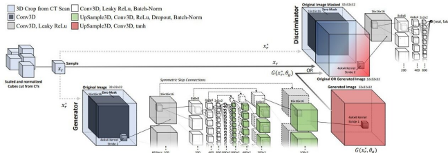
The network architecture, layers, and parameters used for both the injection (GANinj) and removal (GANrem) networks. Credit: arXiv:1901.03597 [cs.CR]
