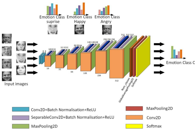
The basic structure of the Light-CNN. Credit: Jie & Yongsheng.
