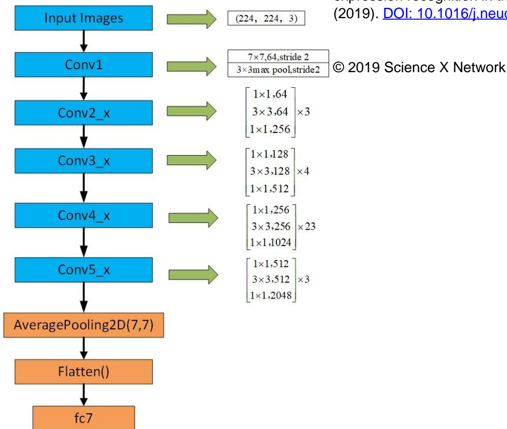
The framework of the pretrained CNN. Credit: Jie & Yongsheng.
