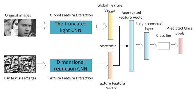
Framework of the dual-branch CNN. Credit: Jie & Yongsheng.
