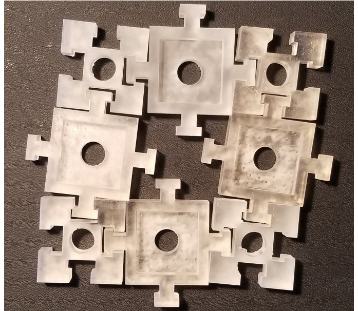
Further examples of the flexibility of planar puzzles. Credit: Lensgraf et al.
