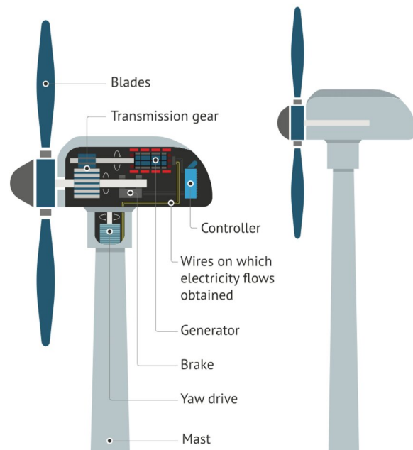
The longer the turbine's blades, the more pressure is put on internal mechanisms. Credit: Shutterstock
