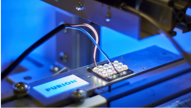
Test set-up for UV-C LEDs. Credit: © Fraunhofer IOSB-AST/Martin Käßler
