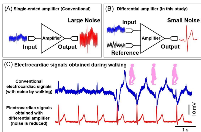
Fig. 1. Electrocardiac signals obtained using flexible organic differential amplifier (A) Conventional single-ended amplifier (B) Differential amplifier developed in this study (C) Electrocardiac signals obtained from a walking subject. In the electrocardiac signals obtained using a conventional single-ended amplifier, large noise caused by walking is included in the waveform. In contrast, such noise is removed from the waveform obtained using the developed flexible organic differential amplifier. Credit: Osaka University
