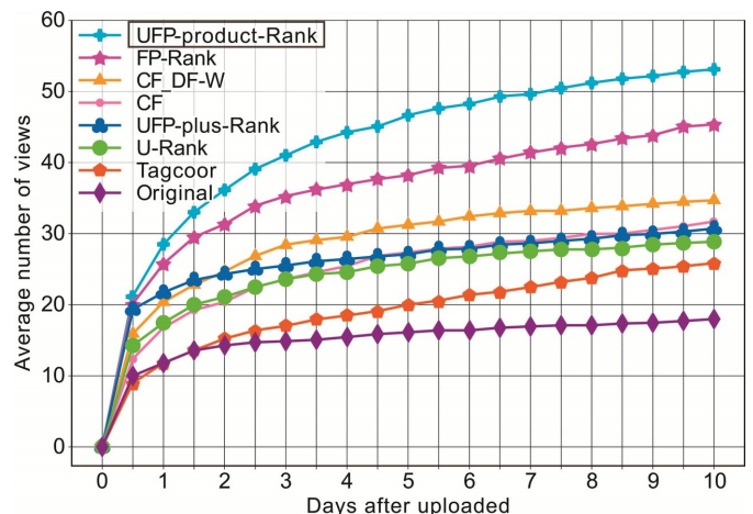
Chart to show popularity of posts that use tags recommended by the algorithm. Credit: Wang et al
