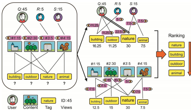
This diagram shows the stages of the algorithm and depicts the way data is used. Credit: Wang et al
