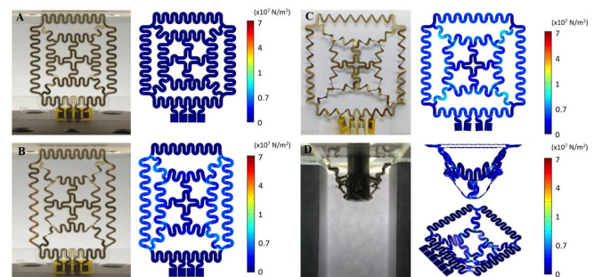
Stability in the skin environment of sensor platform applying complex nature-mimicking structure. Credit: DGIST
