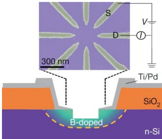
Top view (scanning electron microscopy) and side-view (drawing) of the boron-doped structure. Credit: University of Twente
