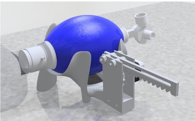
Rack and pinion gear AMBU-bag compression design rendering. Credit: Texas Tech University
