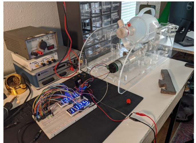
The TTU AMBU-Vent. Credit: Texas Tech University
