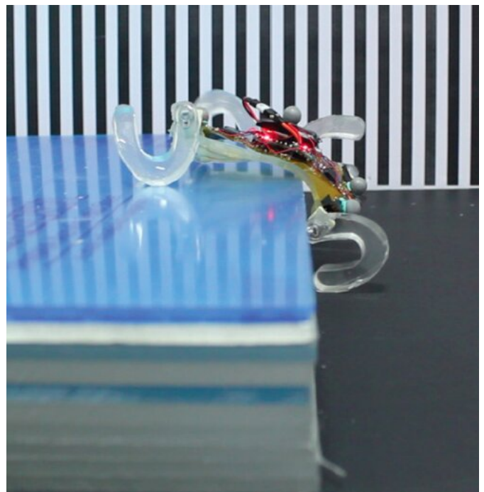
SQuad climbing an object. Credit: Kalin et al.
