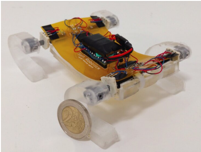
SQuad, the miniature robot developed by the researchers. Credit: Kalin et al.
