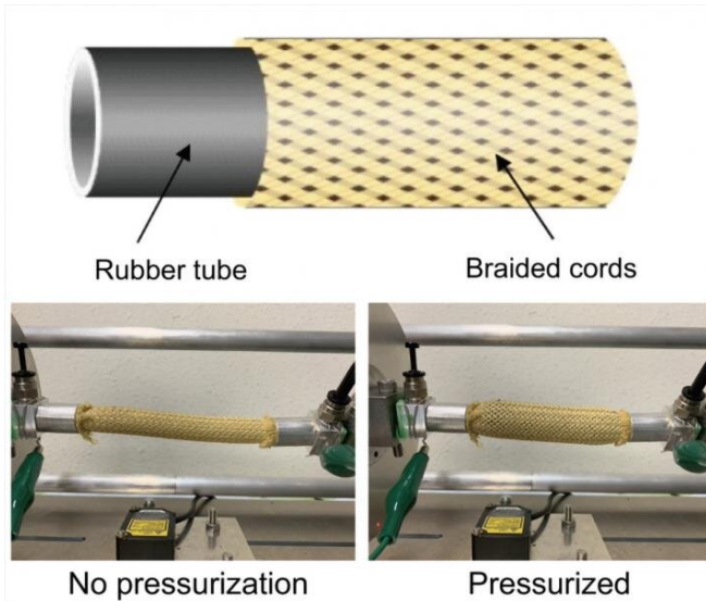
A soft tube expands and contracts to create movement. Credit: © 2020 Nakajima et al.
