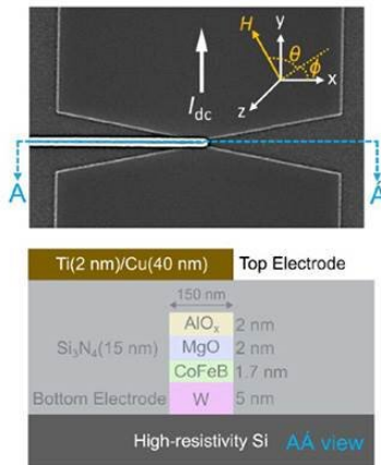
Scanning electron microscopy image and schematic of cross-sectional structure of the created spin-Hall nano-oscillator device with the gate electrode. Credit: Johan Åkerman and Shunsuke Fukami
