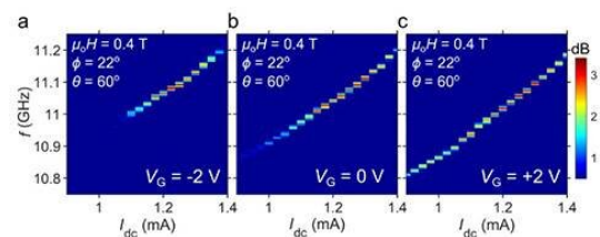
Experimental result of oscillation property under various gate voltages. Red and yellow regions mean a strong oscillation taking place. One can see that the oscillation property changes with the gate voltage. Credit: Johan Åkerman and Shunsuke Fukami
