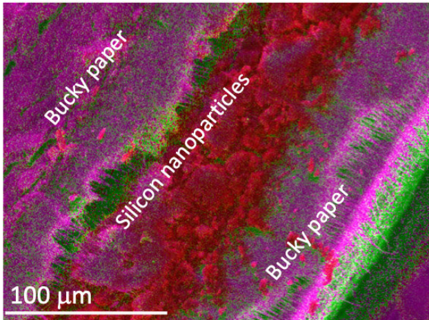
A cross-sectional elemental map shows the microscopic structure of the electrode with silicon nanoparticles. Credit: College of Science
