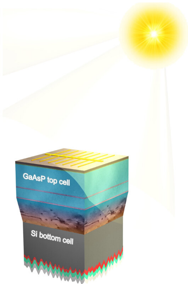
A schematic showing the layered structure of a tandem solar panel. Credit: Mijung Kim
