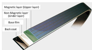
Figure 1: Magnetic tape's layer structure 112
