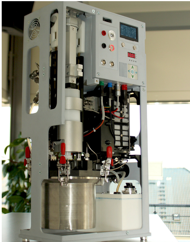
TRL 5 demonstrator of a power generator with a POWERPASTE cartridge and a 100 watt PEM fuel cell. Credit: Fraunhofer-Gesellschaft
