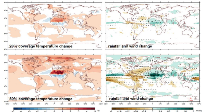
Global temperature, rainfall and surface wind changes in simulations with 20% and 50% solar panel coverage of Sahara. Credit: Lu et al. (2021) , Author provided
