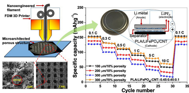
Graphical abstract. Credit: Journal of Power Sources (2021). DOI: 10.1016/j.jpowsour.2021.229625
