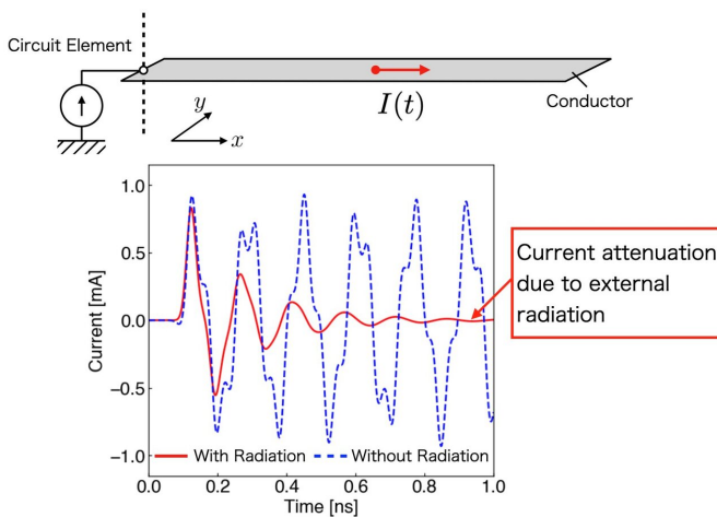
Fig. 3 Effect of radiation on conducted signals: The red line shows the calculation result with external radiation obtained by the newly developed method, while the blue line shows the calculation result ignoring the radiation by approximating the delay time as zero. The waveform in the graph shows the time variation of the current flowing in the center of the conductor, and its oscillation shows the input pulse current propagating through the conductor, bouncing back and forth at both ends. Credit: Osaka University
