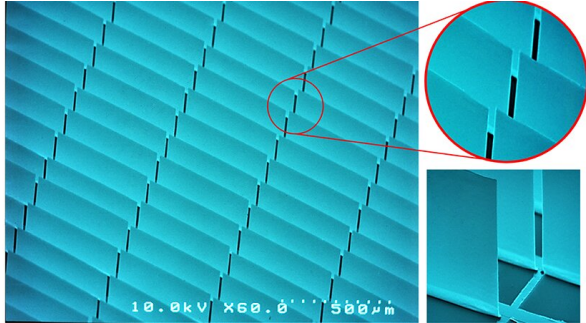
SEM micrograph of vertically standing, flat micromirror array with an inset of magnified area. Credit: Hillmer et al.
