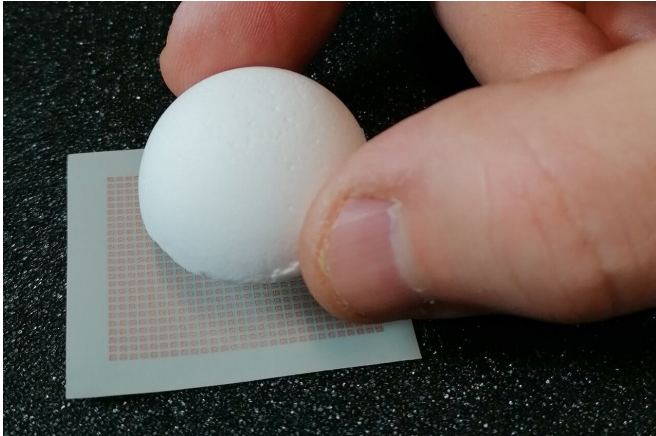
Composite lens made of nanocellulose for 6G frequency, about 800 antennas. Credit: University of Oulu
