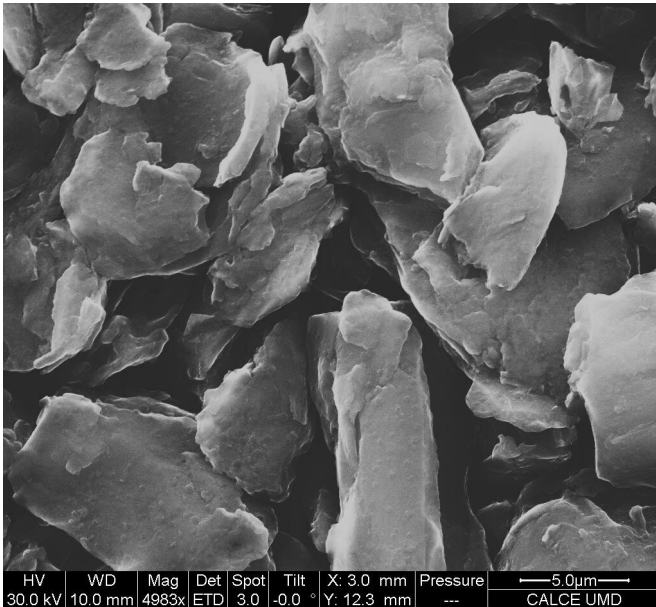
SEM of anode. Credit: Heriot-Watt University
