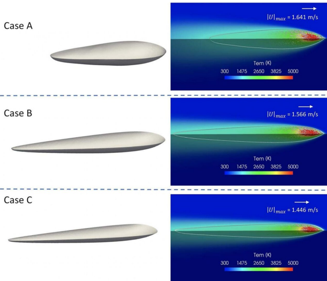
Melt pool shape and the temperature and melt pool flow velocity predicted by a physics-informed neural network (PINN) for case A, B and C at quasi-steady state (2 microseconds). Credit: Qiming Zhu, Zeliang Liu, Jinhui Yan
