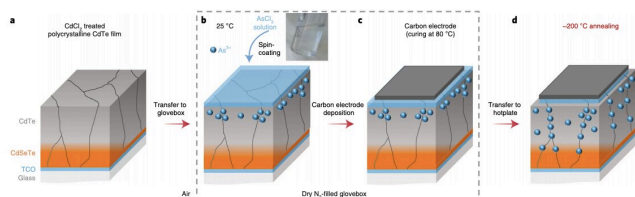
Schematic figure representing low-temperature ex situ doping of polycrystalline CdSeTe solar cells. Credit: Li et al.
