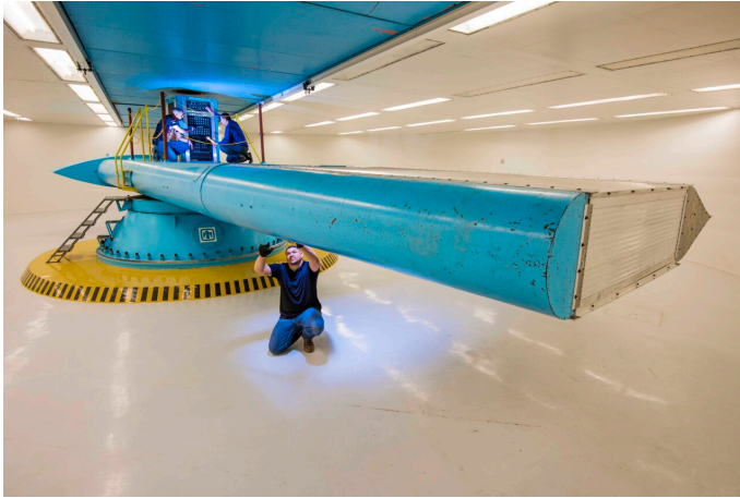
The Sandia National Laboratories Superfuge/Centrifuge Complex aims to provide the most realistic flight simulation environments possible. Credit: Randy Montoya
