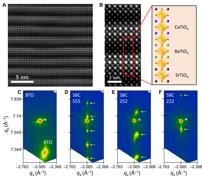
Structural characterization of superlattices. (A) Cross-sectional STEM acquired from sample SBC222. (B) High-resolution STEM from a part of the scanned region. The schematic depicts the arrangement of unit cells. RSM acquired around (103) reflection in (C) BTO, (D) SBC555, (E) SBC252, and (F) SBC222. Star and yellow arrows indicate the STO substrate and satellite peaks from SL, respectively. Credit: Science Advances (2021). DOI: 10.1126/sciadv.abe4206
