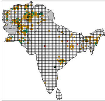
IMAGE: SNAPSHOT OF A WEEKLY PREDICTION OF NON-STATE TERRORISM IN GRID CELLS (50 KM X 50 KM) ACROSS SOUTH ASIA (■ TRUE POSITIVE; □ TRUE NEGATIVE; ■ FALSE POSITIVE; ■ FALSE NEGATIVE). CREDIT: ANDRE PYTHON (2021)
