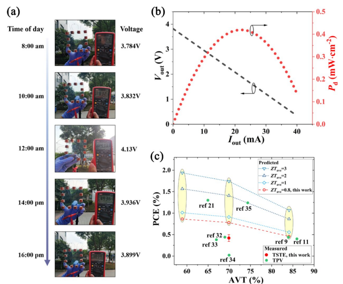
Fig. 2 Power-generating performance of a typical solar-thermal-electric power-generating window. Credit:
