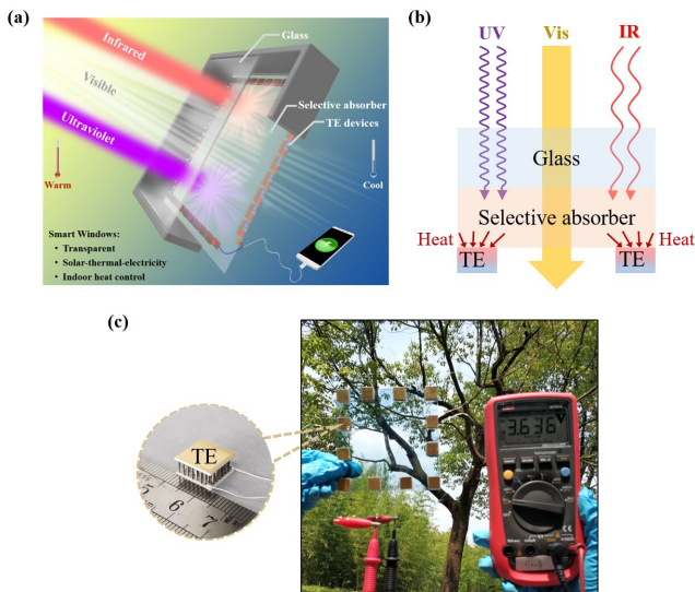
Fig. 1 Schematic diagram and demonstration of energy-saving power window technology based on solar-thermal-electric conversion. Credit: SICCAS
