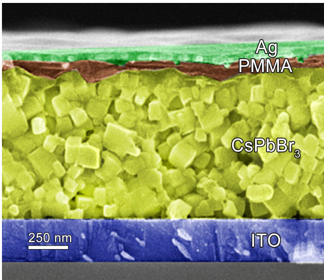
A scanning electron microscope image of the light emitting memory, with each key layer labeled. Credit: Kyushu University/Ya-Ju Lee
