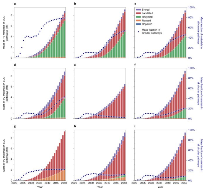
Fig. 1: Various interventions could improve material circularity in the PV sector. a–i, Landfill ban (a), high material recovery (96%) and US $18 per module recycling costs (b), lower recycling costs (US $18 per module) (c), higher landfill costs (US $2.75 per module) (d), improved learning (from 30 to 60 yr in 2050) (e), improved learning effect (learning parameter = 0.6) (f), reuse warranties (equal new/used attitude) (g), seeding reuse (5% of population per year) (h) and baseline (i). Some interventions, which include improved warranties (g) and seeding used modules (h), particularly boost module repair and reuse. Other interventions, such as lower initial recycling costs (c) and higher landfill costs (d), boost recycling. Credit: DOI: 10.1038/s41560-021-00888-5
