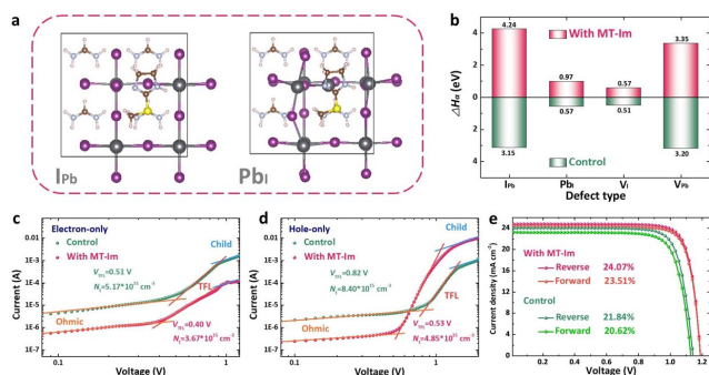
a. Theoretical calculation model; b. the formation energy (?H?) of interface defects; c,d. Defect density calculation and photovoltaic performance test of perovskite solar cells. Credit: Liu Guozhen.
