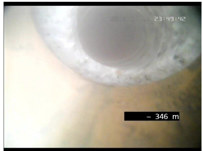
View of a freshly drilled side arm at 346 meters. The micro drilling turbine milled out the granite rock cleanly. Credit: Fraunhofer-Gesellschaft
