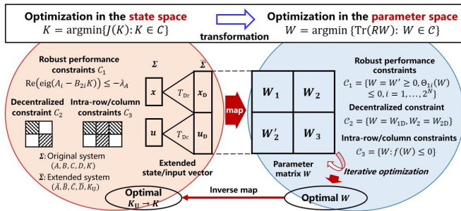
The schematic illustration of the proposed structured optimal control method. Credit: NIMTE
