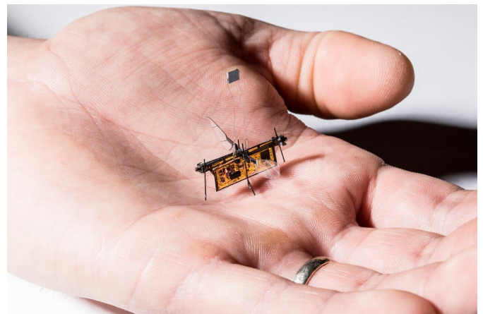
The first wireless flying robotic insect takes off. Credit: Sawyer Fuller
