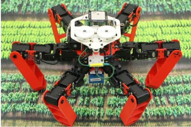
A walking robot that uses sky polarization for navigation. Credit: Julien Dupeyroux
