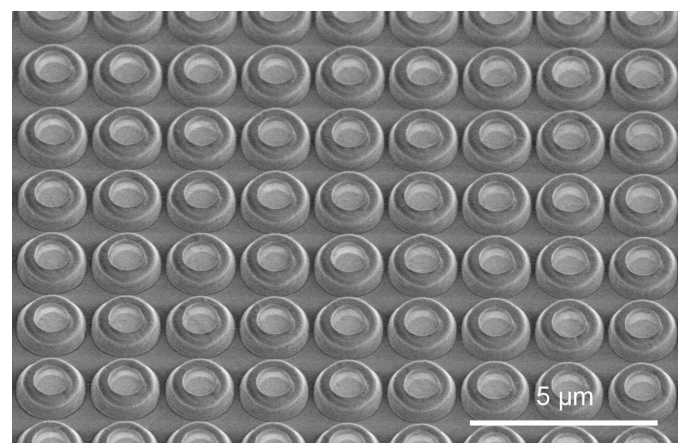
Electron micrograph of an array of UV micro-LEDs with 2 \mu\text{m} pitch. Credit: FBH
